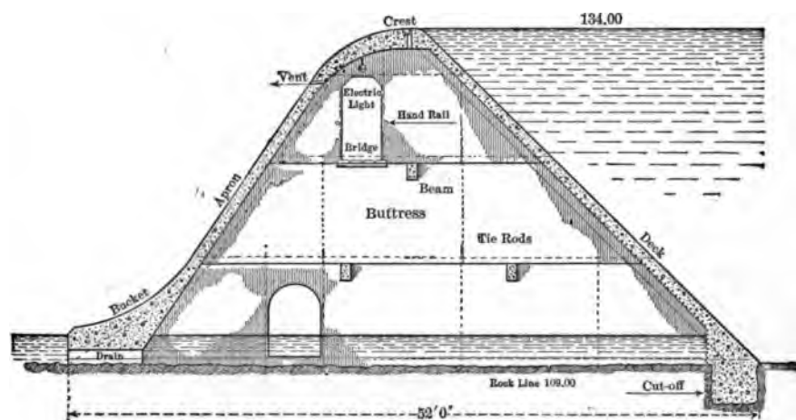
FIG. 49.—SCHUYLERVILLE DAM.
