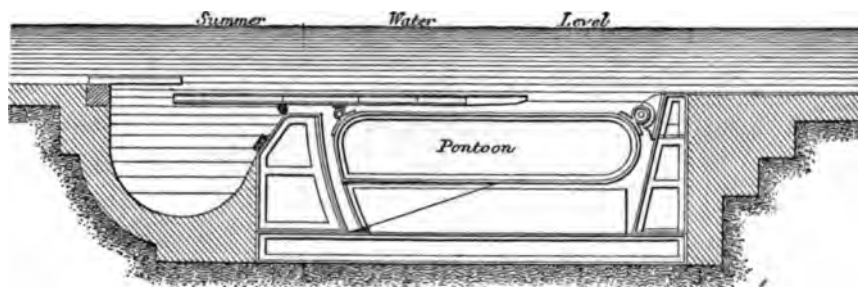
FIG. 100.—KRANTZ PONTOON-DAM.
