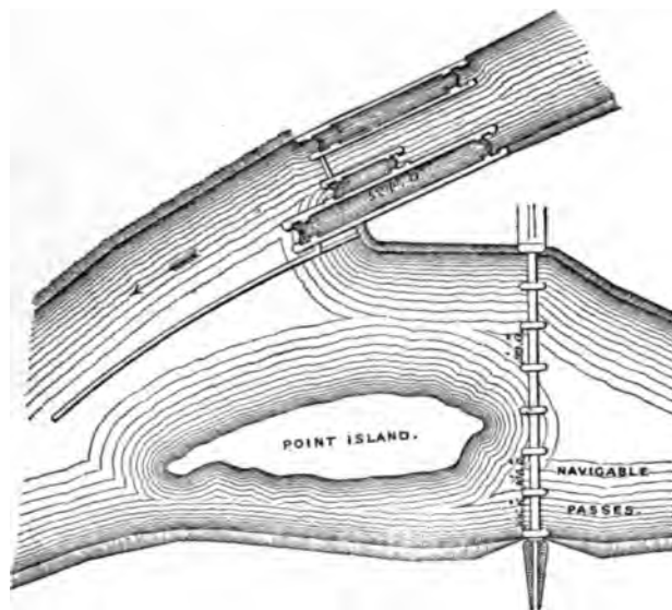
FIG. 89.—POSES DAM.
