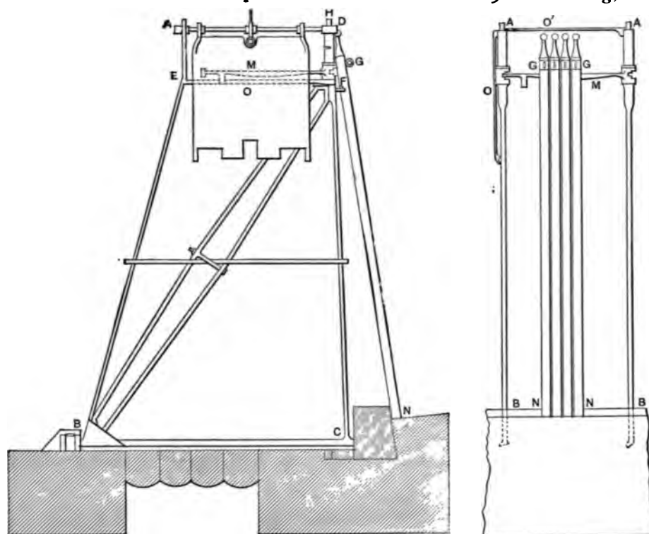
FIG. 81.—BELGIAN NEEDLE-DAM.
