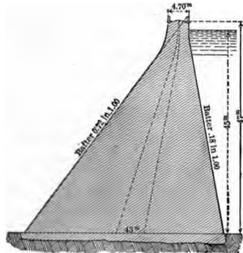
FIG. 29.—THE CHER DAM.
