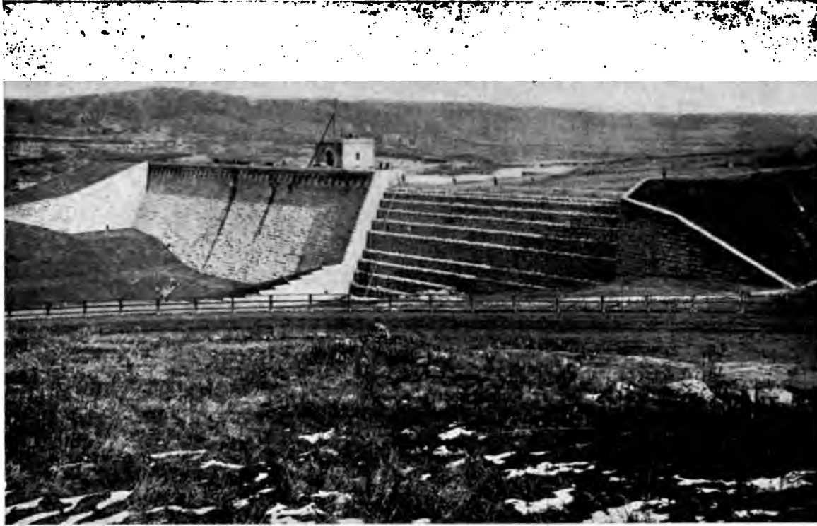
TITICUS DAM, FRONT FACE.
