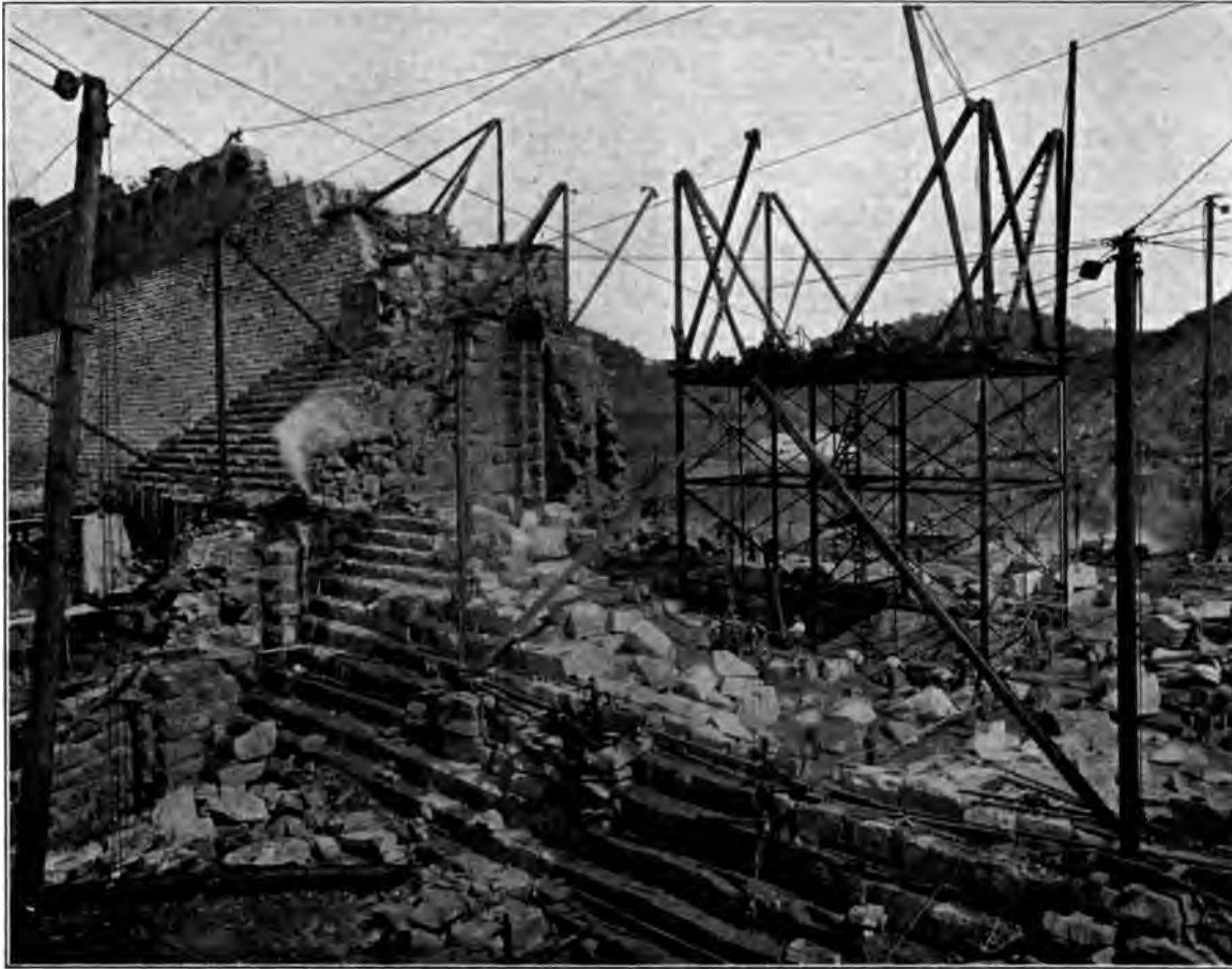
NEW CROTON DAM. DERRICK PLATFORM.
