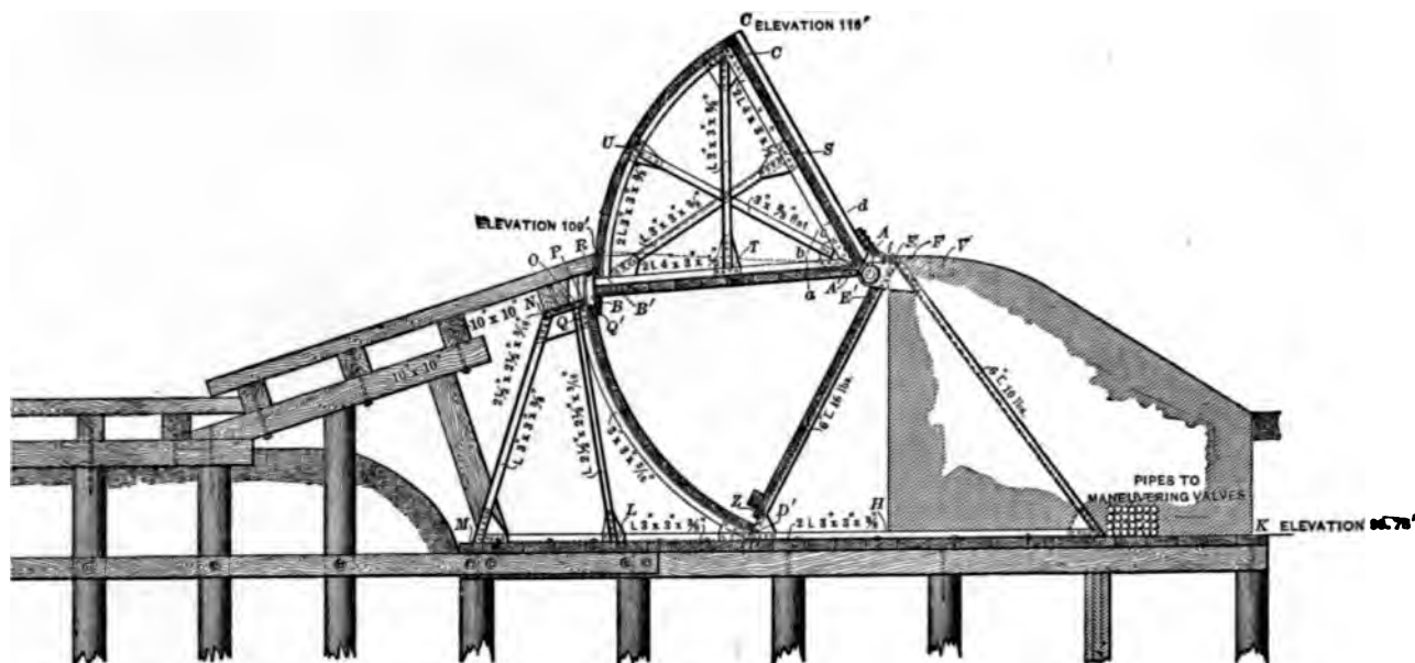
FIG. 106.—CHITTENDEN DRUM-DAM.
