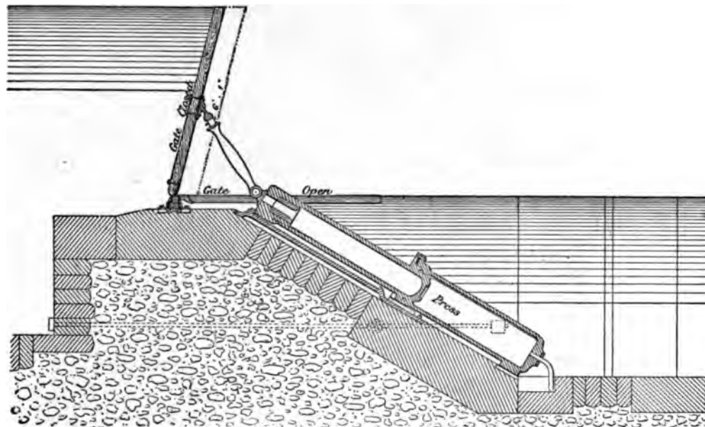
FIG. 102.—GIRARD SHUTTER-DAM.
