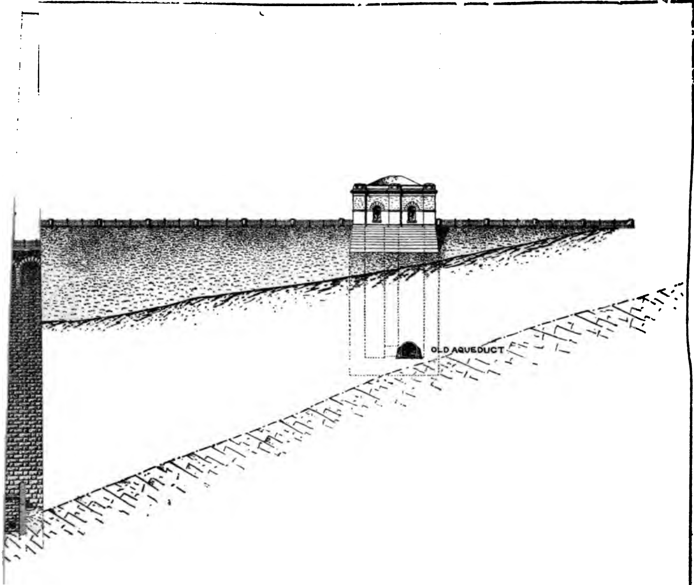
THE AQUEDUCT COMMISSIONERS NEW CROTON DAM AT CORNELL SITE
