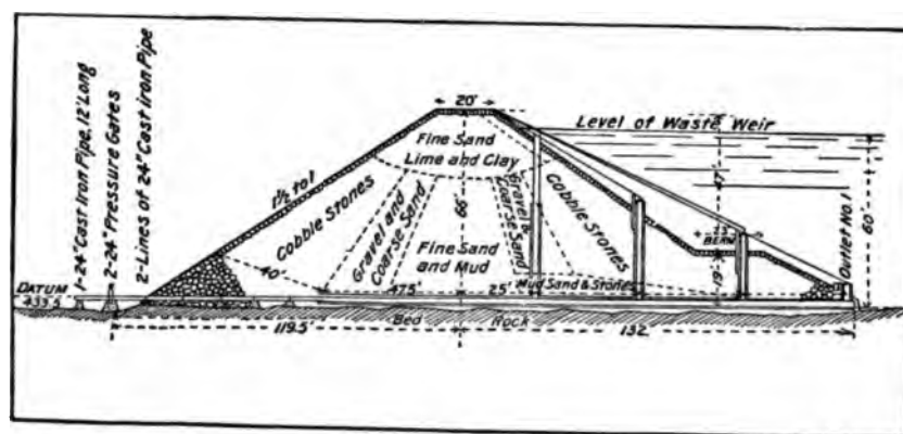
FIG 57.—CROSS-SECTION OF LA MESA DAM.
