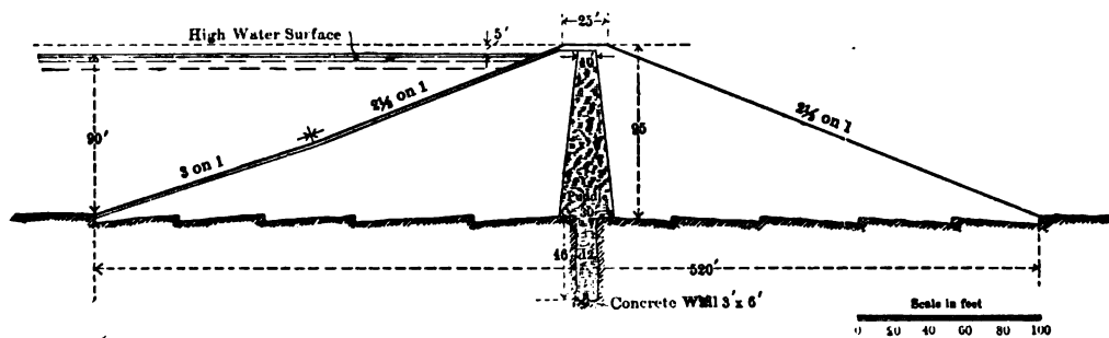
FIG. 54.†—CROSS-SECTION OF PILARCITOS DAM.
