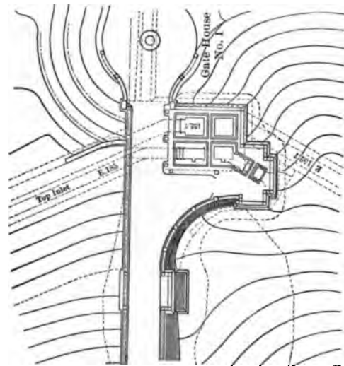
FIG. 36.—GATE-HOUSE NO. 1.
