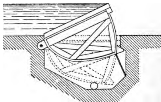
BRUNOT GATE.
