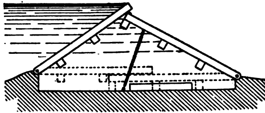
FIG. 107.—BEAR-TRAP GATE, DAVIS ISLAND DAM.
