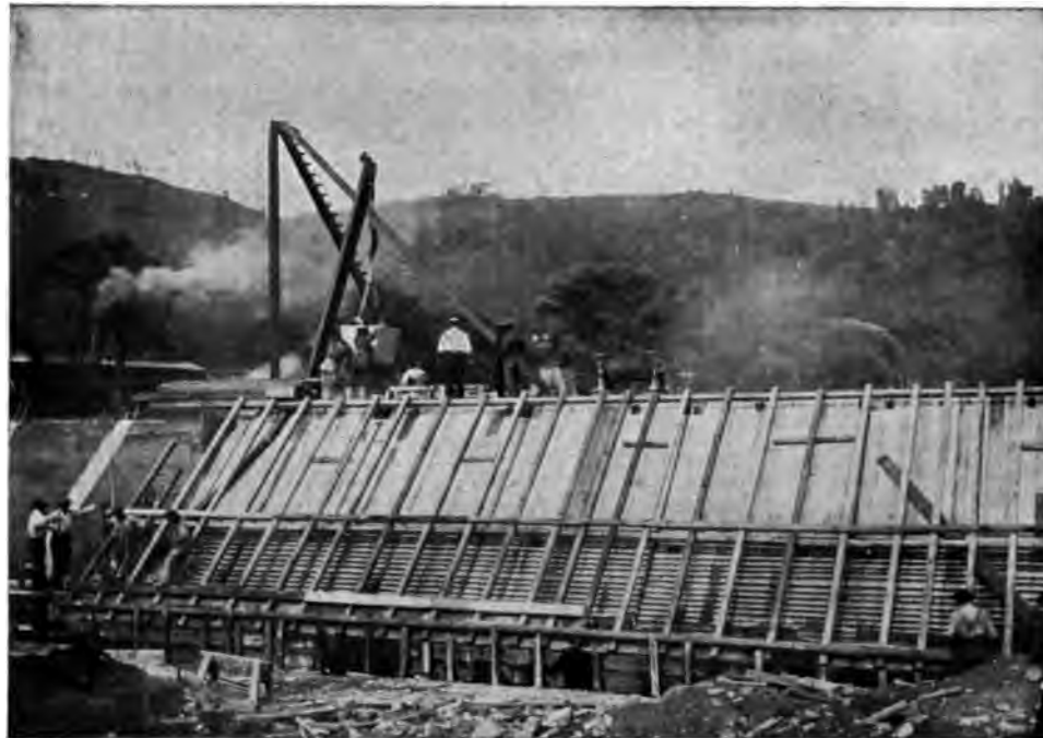
JUNIATA DAM. CONSTRUCTING DECK OF REINFORCED CONCRETE.
