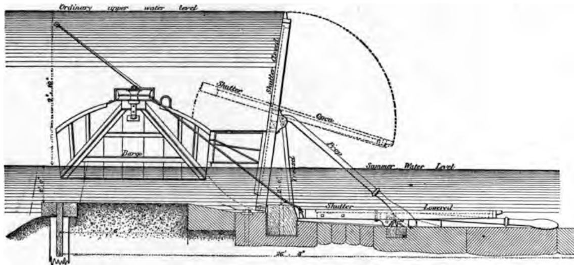
FIG. 94.—CHANOINE SHUTTER-DAM ON NAVIGABLE PASS ON THE UPPER SEINE.
