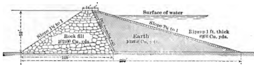
FIG. 64.—PECOS VALLEY DAM. NO. 2.
