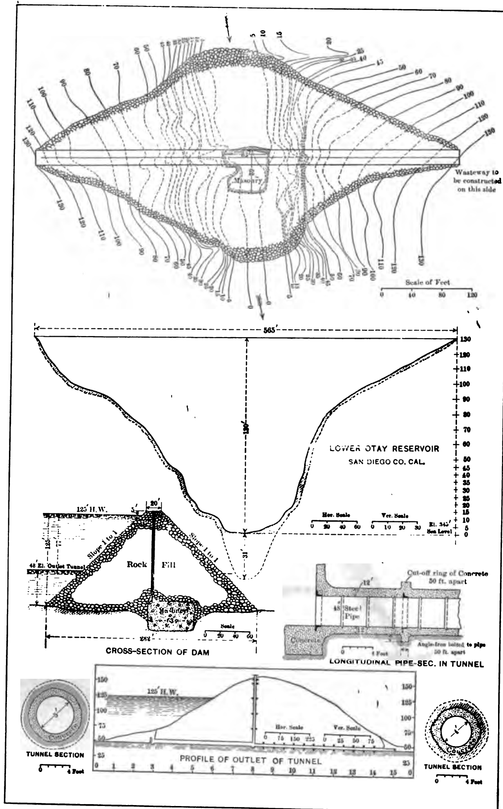
LOWER OTAY DAM.
