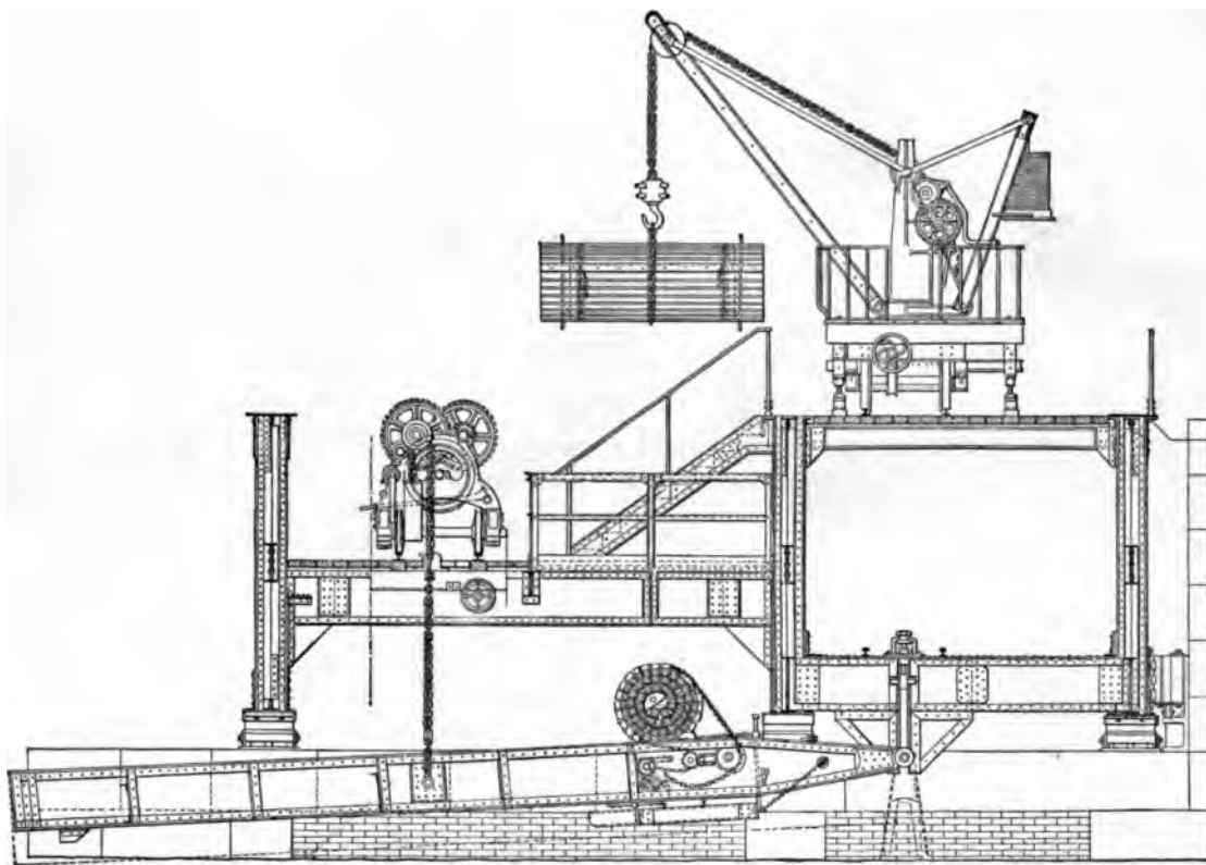
FIG. 88.—CROSS-SECTION OF CAMÉRE CURTAIN-DAM.
