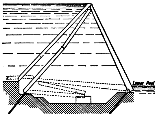
FIG. 114.—PARKER GATE.
