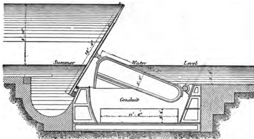
FIG. 99.—KRANTZ PONTOON-DAM.
