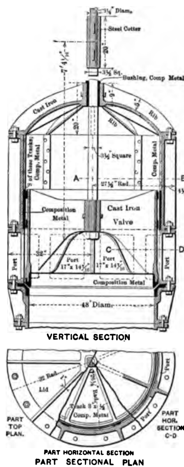
FIG. 38.—BALANCED VALVE.
