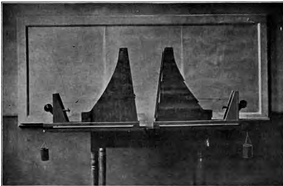
FIG. 5.—ATCHERLEY'S MODELS OF DAMS.
