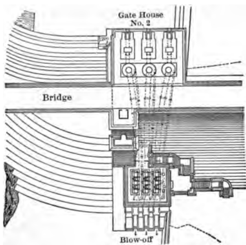
FIG. 37.—GATE-HOUSE No. 2.
