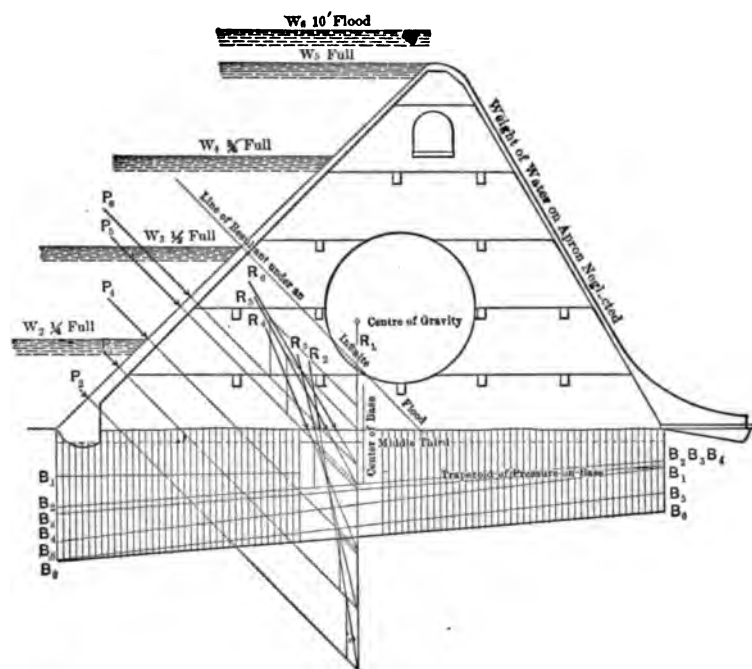
FIG. 48.—PROFILE FOR CONCRETE-STEEL DAM.
