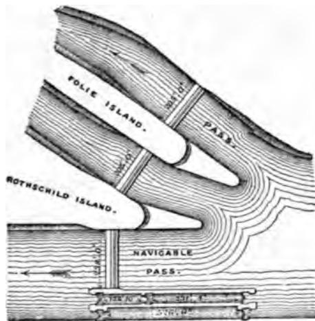
FIG. 91.—SURESNES DAM.
