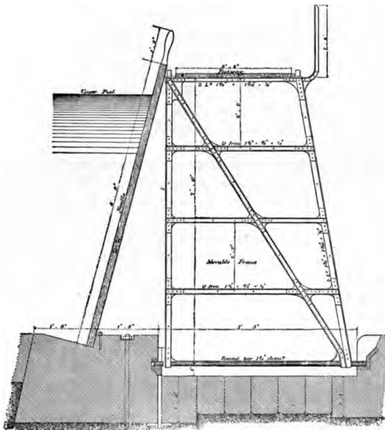
FIG. 80.—POIRÉE NEEDLE-DAM.
