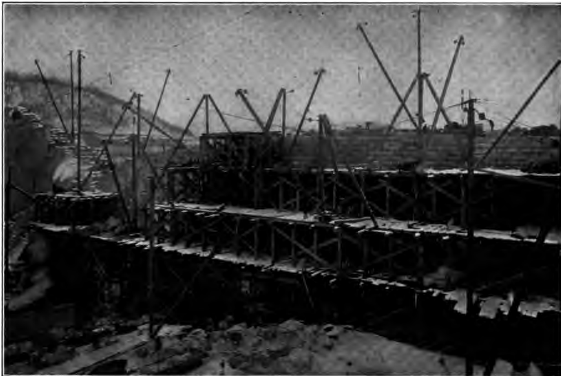
NEW CROTON DAM. TRESTLE ON DOWN-STREAM FACE.
