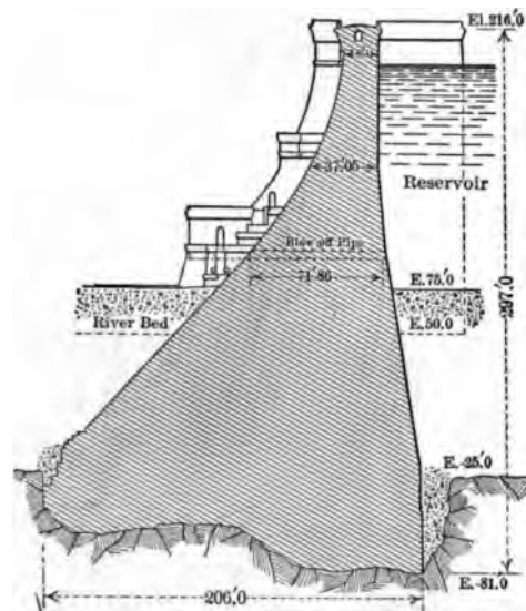
FIG. 35.—MAXIMUM SECTION.
