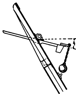
FIG. 101.—BUTTERFLY VALVE.
