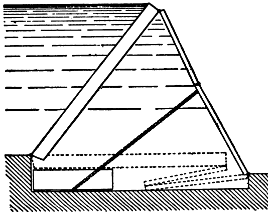
FIG. 111.—GIRARD GATE.
