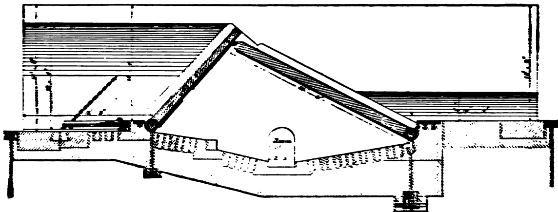
FIG. 103.—BEAR-TRAP DAM ON THE MARNE.
